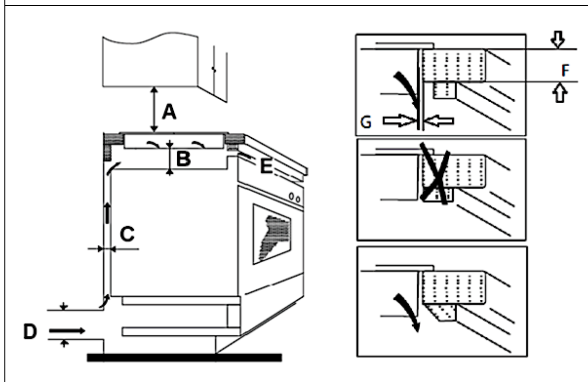
C = VENTILATION SLOT
