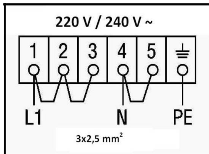
Connection diagram
