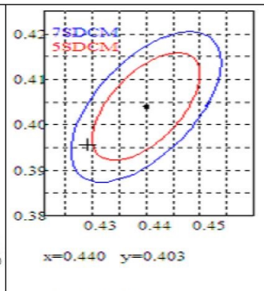
SDCM=5.5 SDCM Color Difference Chart
